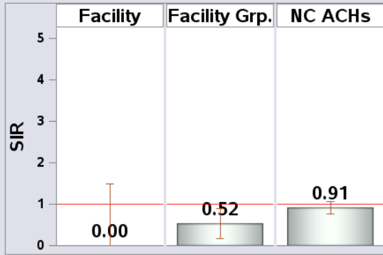
Figure 4: SIRs and 95% confidence intervals, Jan-Mar 2018.
