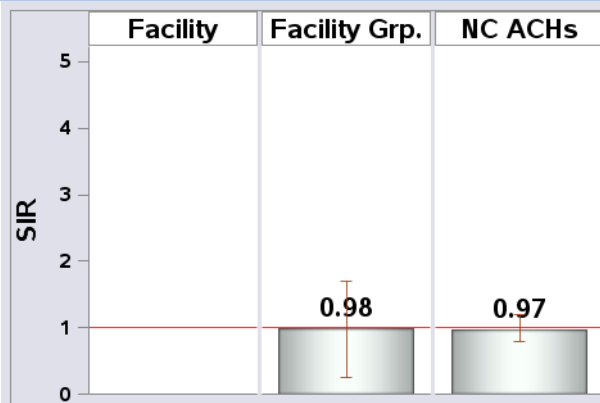
Figure 2: SIRs and 95% Confidence Intervals, Jan-Mar 2018.
