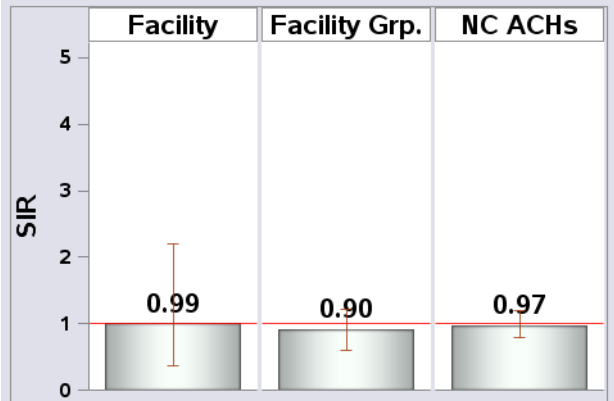
Figure 2: SIRs and 95% Confidence Intervals, Jan-Mar 2018.
