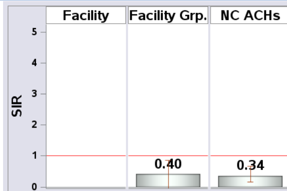
Figure 5: SIRs and 95% Confidence Intervals, Jan-Mar 2018.
