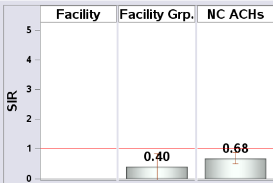
Figure 6: SIRs and 95% Confidence Intervals, Jan-Mar 2018.
