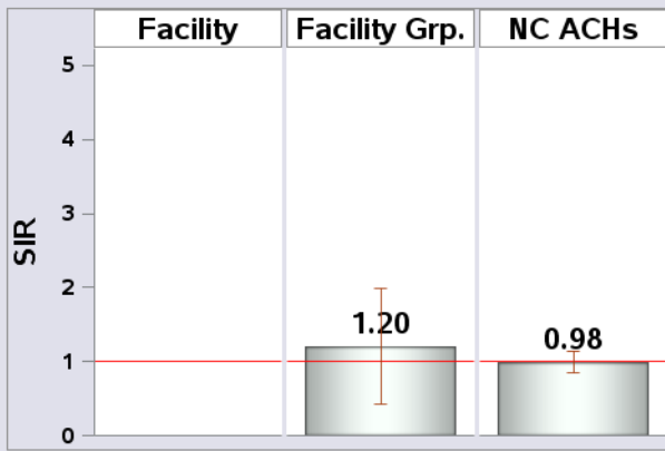
Figure 1: SIRs and 95% confidence intervals, Jan-Mar 2018.
