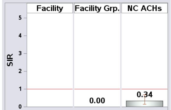
Figure 5: SIRs and 95% Confidence Intervals, Jan-Mar 2018.
