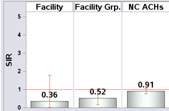
Figure 4: SIRs and 95% confidence intervals, Jan-Mar 2018.
