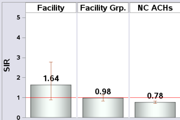
Figure 3: SIRs and 95% Confidence Intervals, Jan-Mar 2018.
