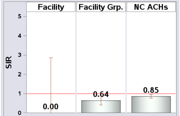
Figure 2: SIRs and 95% Confidence Intervals, Jan-Dec 2018.
