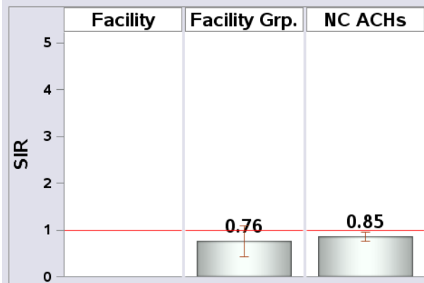
Figure 2: SIRs and 95% Confidence Intervals, Jan-Dec 2018.
