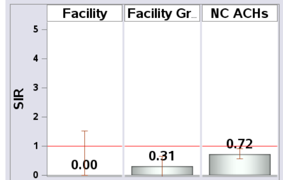
Figure 5: SIRs and 95% Confidence Intervals, Jan-Dec 2018.
