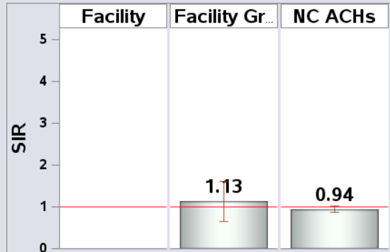
Figure 4: SIRs and 95% confidence intervals, Jan-Dec 2018.
