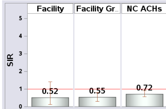
Figure 5: SIRs and 95% Confidence Intervals, Jan-Dec 2018.
