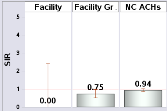
Figure 4: SIRs and 95% confidence intervals, Jan-Dec 2018.
