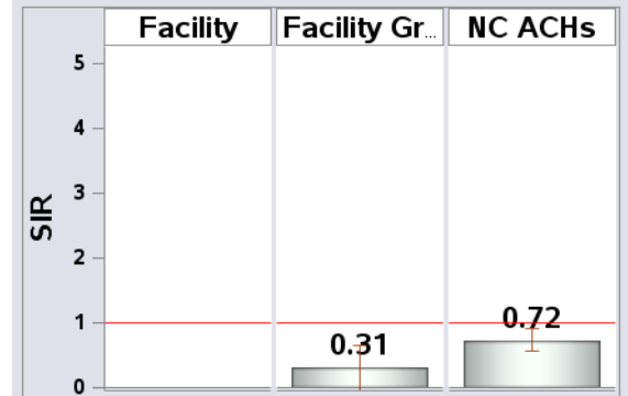
Figure 5: SIRs and 95% Confidence Intervals, Jan-Dec 2018.
