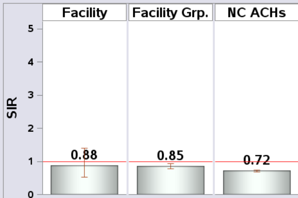
Figure 3: SIRs and 95% Confidence Intervals, Jan-Dec 2018.
