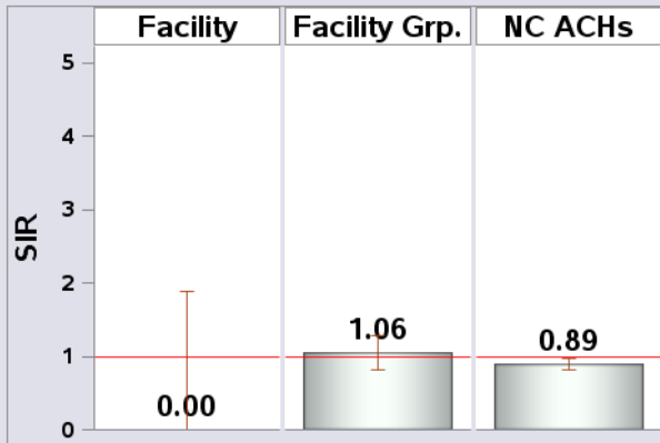
Figure 1: SIRs and 95% confidence intervals, Jan-Dec 2018.
