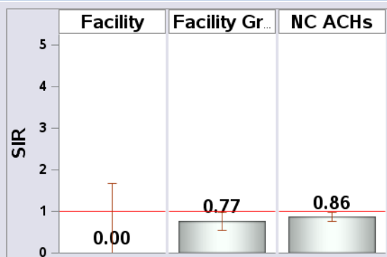
Figure 6: SIRs and 95% Confidence Intervals, Jan-Dec 2018.
