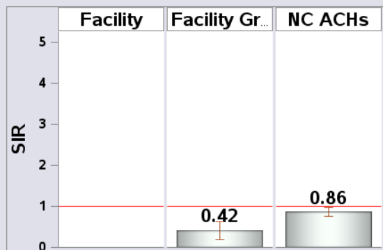
Figure 6: SIRs and 95% Confidence Intervals, Jan-Dec 2018.
